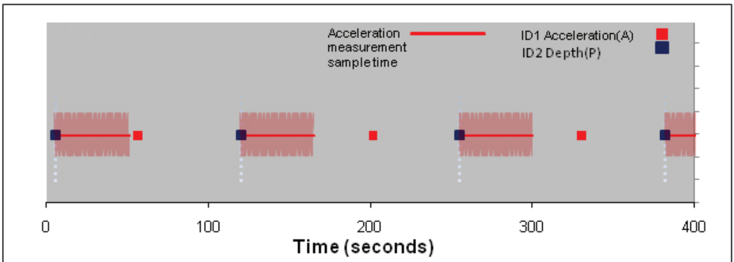
Figure 3: Example of sampling and transmission format for the V13AP. For the V13A, acceleration would be sampled for every delay cycle.
